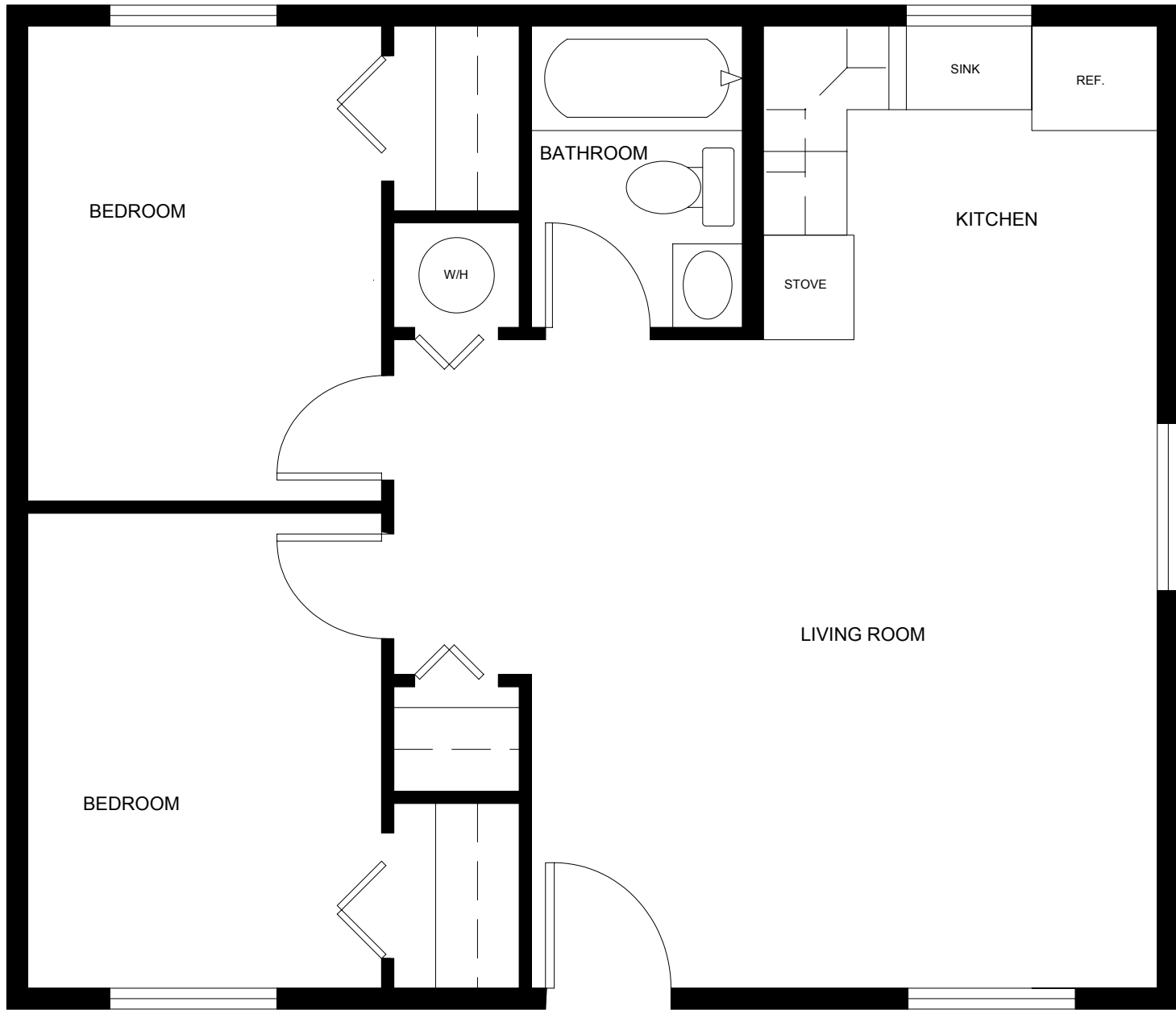
28'x24' TYPICAL (DOUBLE) NOT TO SCALE
